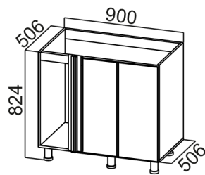
M1000y(400)*** 1. 900x824x506 2. 1000x850x600
