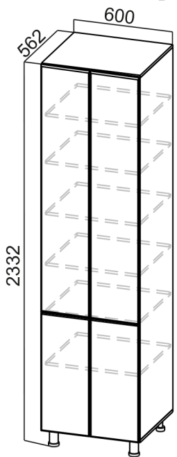
П600г (600x2332x562)
