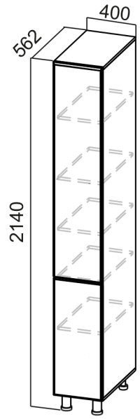
П400г (400x2140x562)
