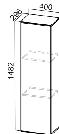
ПН400(912/296) (400x1482x296)
