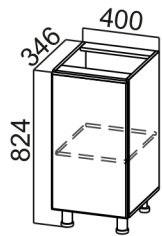
C400(400)*** 1. 400x824x346 2. 400x850x400
