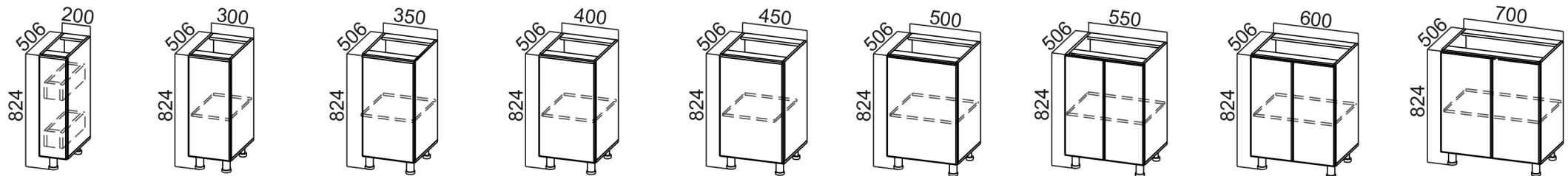
C2006*** 1. 200x824x506 2. 200x850x600 C300*** 1. 300x824x506 2. 300x850x600 C350*** 1. 350x824x506 2. 350x850x600 C400*** 1. 400x824x506 2. 400x850x600 C450*** 1. 450x824x506 2. 450x850x600 C500*** 1. 500x824x506 2. 500x850x600 C550*** 1. 550x824x506 2. 550x850x600 C600*** 1. 600x824x506 2. 600x850x600 C700*** 1. 700x824x506 2. 700x850x600
