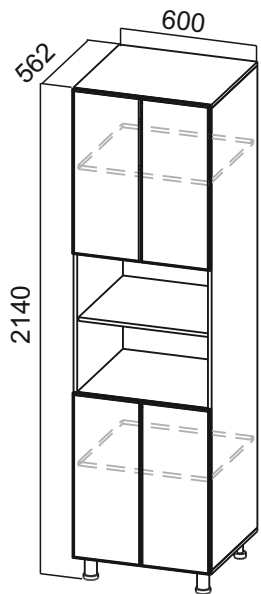
П600 (600x2140x562)
